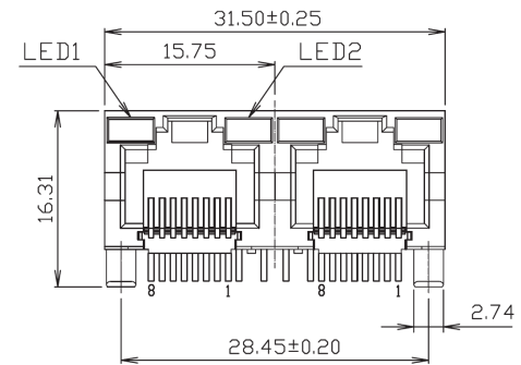
RIA Connector P/N: AJT35I8821-030
